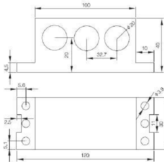
Current Transformer (0.1A-100A)
