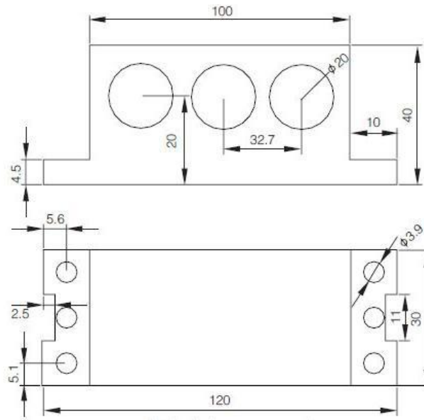
Figure 3 Transformer mounting dimension of less than 100A
