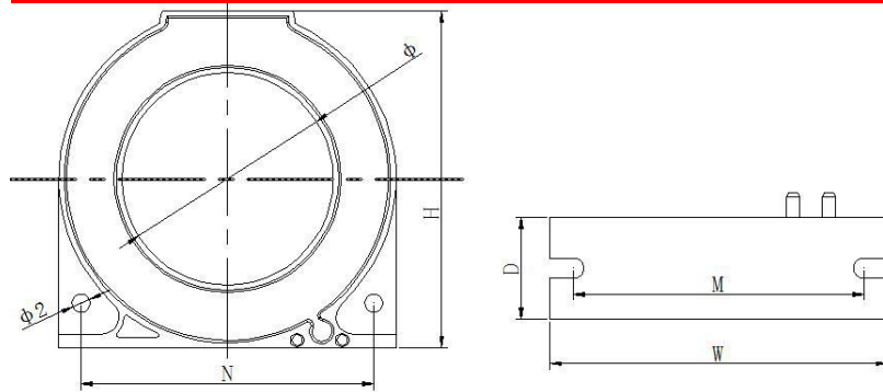
Figure 5 outline dimensions of outlay current transformer
