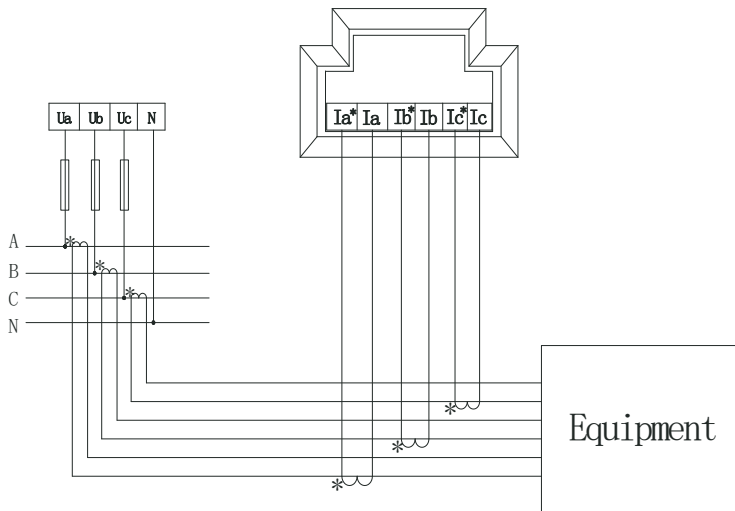
Picture 7 Three-phase four-wire (secondary current access)
