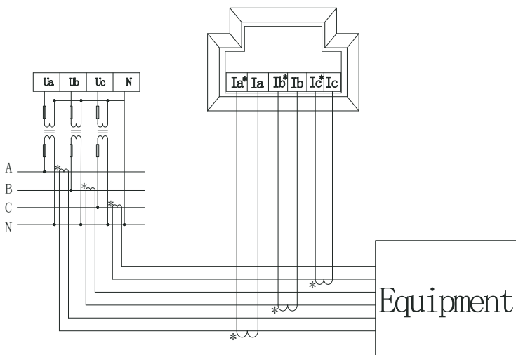
Picture 9 Three-phase four-wire (secondary connection of voltage and current)
