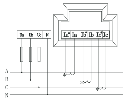
Picture 8 Three-phase four-wire (direct current connection)
